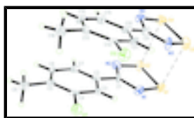
Fig. 1. The structure of the title compound with displacement ellipsoids drawn at the 50% probability level showing S...S contacts (dashed lines).
